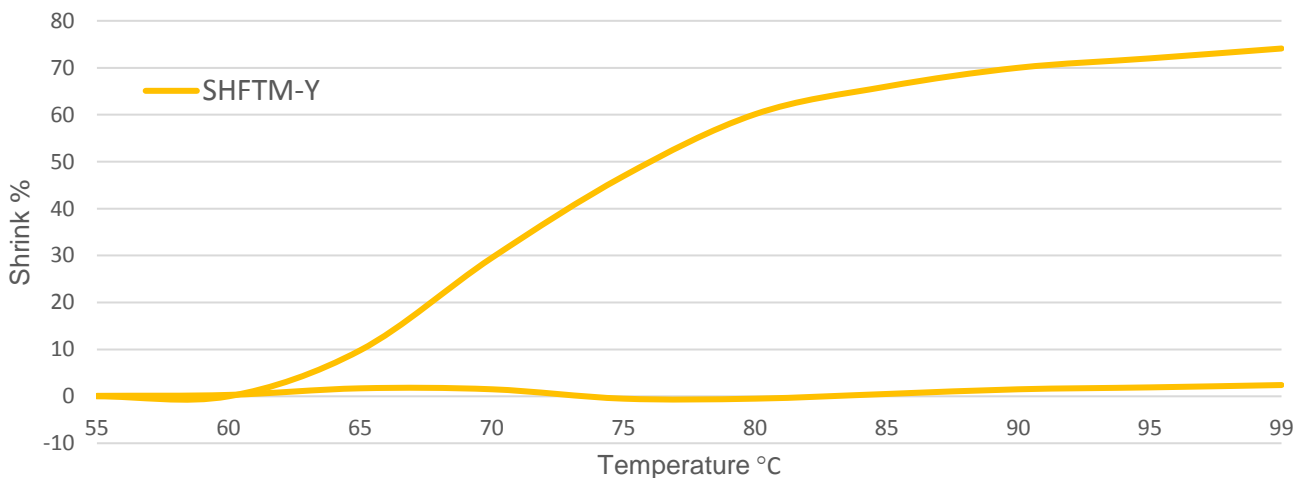
TD and MD Shrink curves
